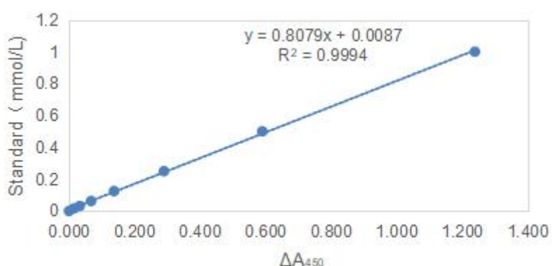
Figure 1. Standard curve of cellulase activity assay.
